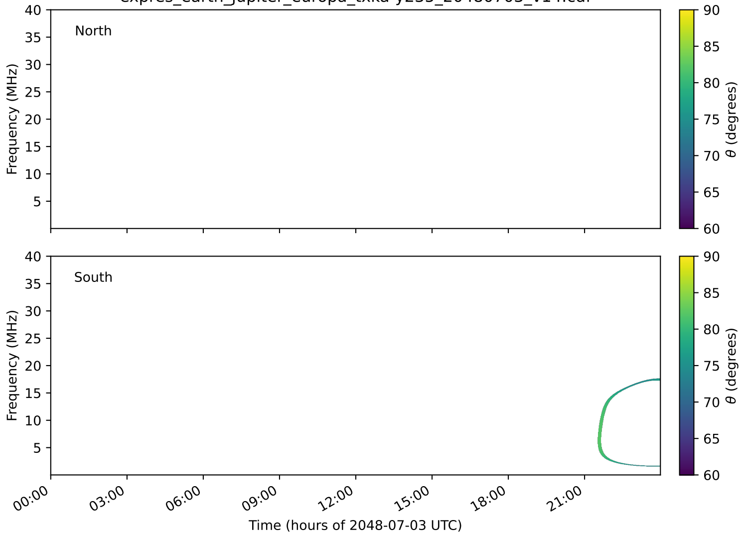
expres_earth_jupiter_europa_txka-y235_20480703_v14.cdf
