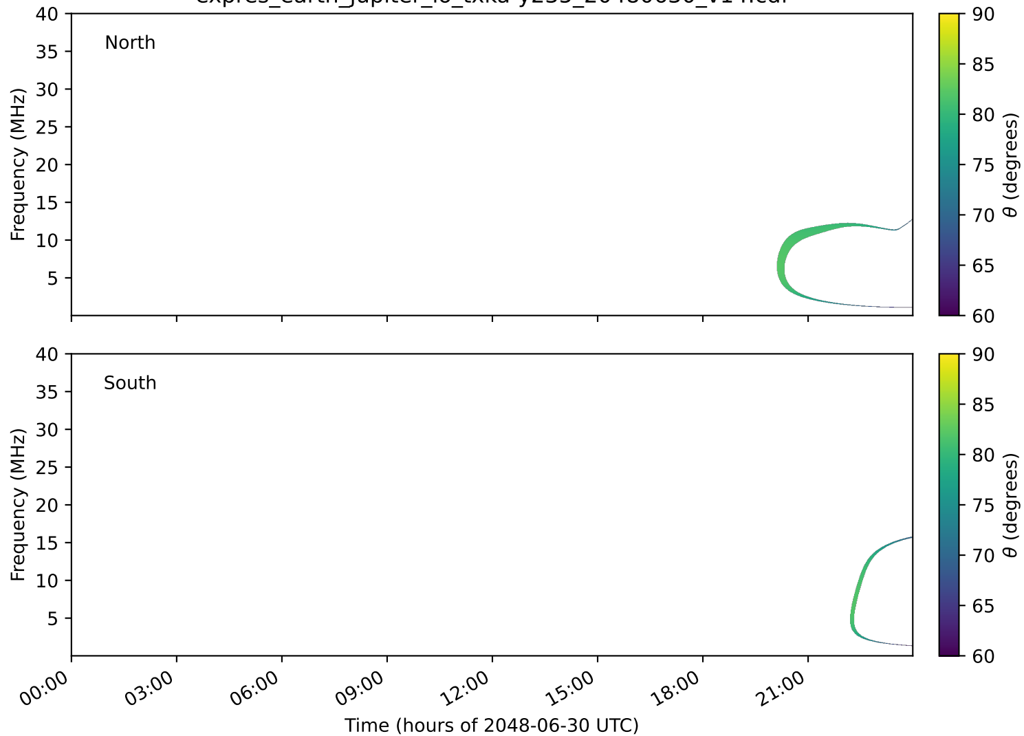
expres_earth_jupiter_io_txka-y235_20480630_v14.cdf
