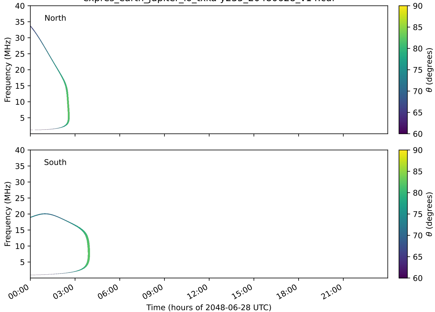
expres_earth_jupiter_io_txka-y235_20480628_v14.cdf
