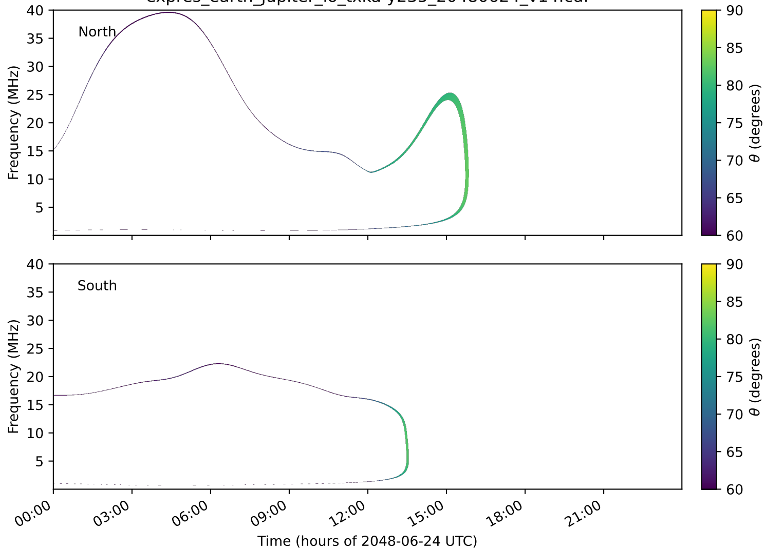
expres_earth_jupiter_io_txka-y235_20480624_v14.cdf
