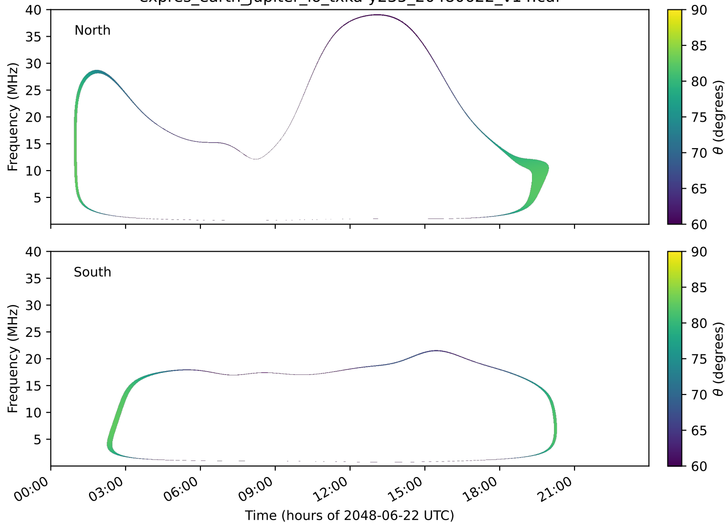
expres_earth_jupiter_io_txka-y235_20480622_v14.cdf
