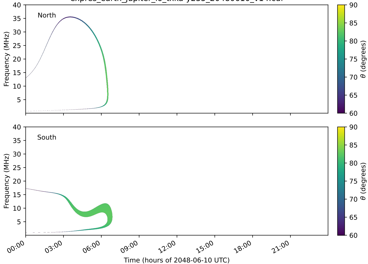
expres_earth_jupiter_io_txka-y235_20480610_v14.cdf
