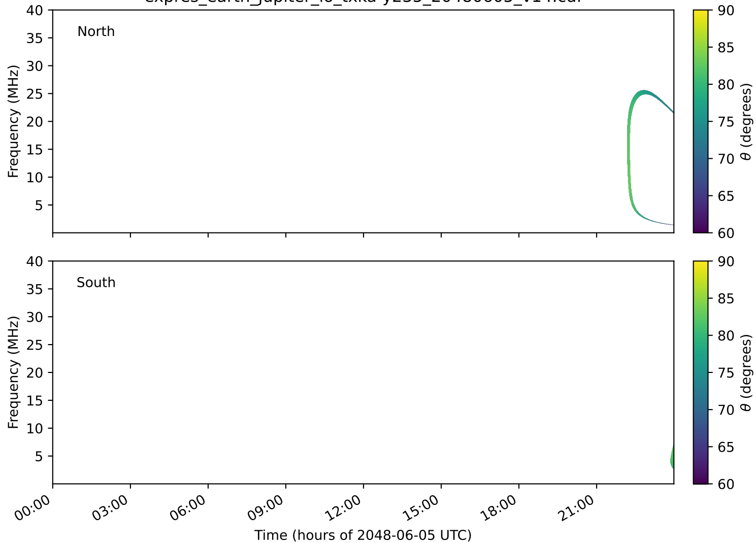
expres_earth_jupiter_io_txka-y235_20480605_v14.cdf
