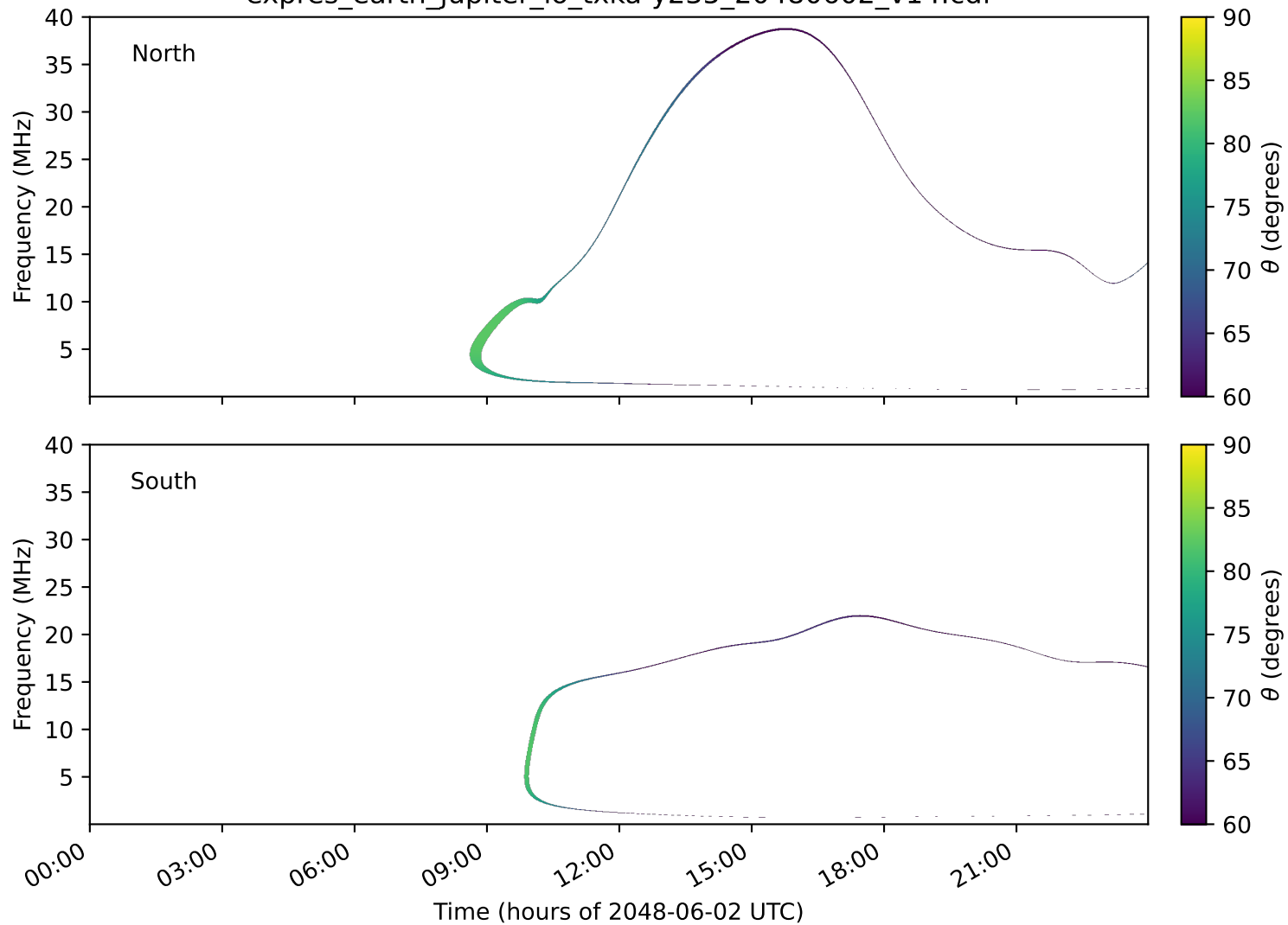
expres_earth_jupiter_io_txka-y235_20480602_v14.cdf
