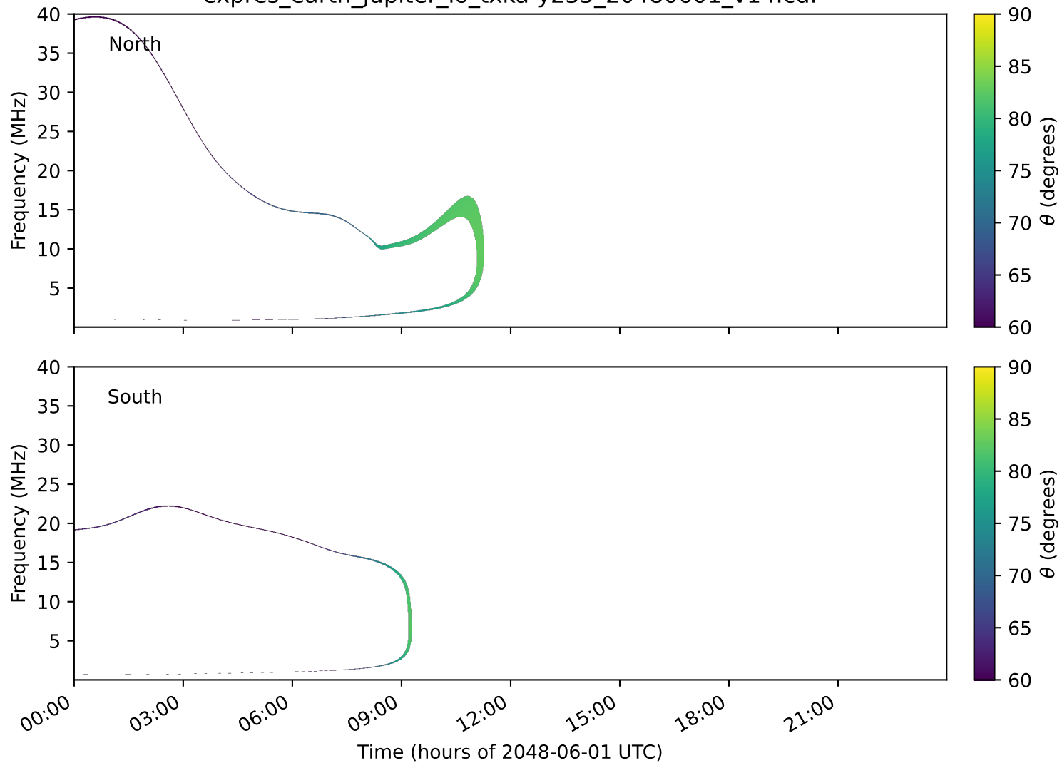
expres_earth_jupiter_io_txka-y235_20480601_v14.cdf
