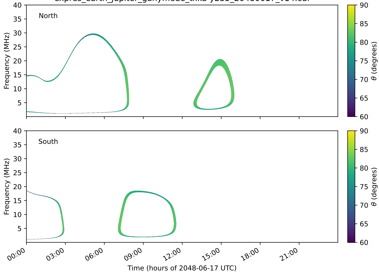
expres_earth_jupiter_ganymede_txka-y235_20480617_v14.cdf
