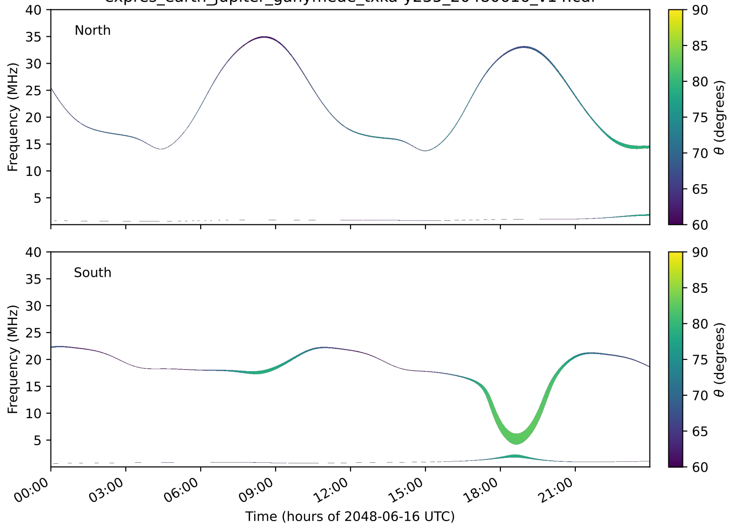
expres_earth_jupiter_ganymede_txka-y235_20480616_v14.cdf
