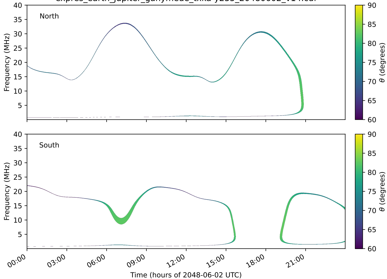
expres_earth_jupiter_ganymede_txka-y235_20480602_v14.cdf
