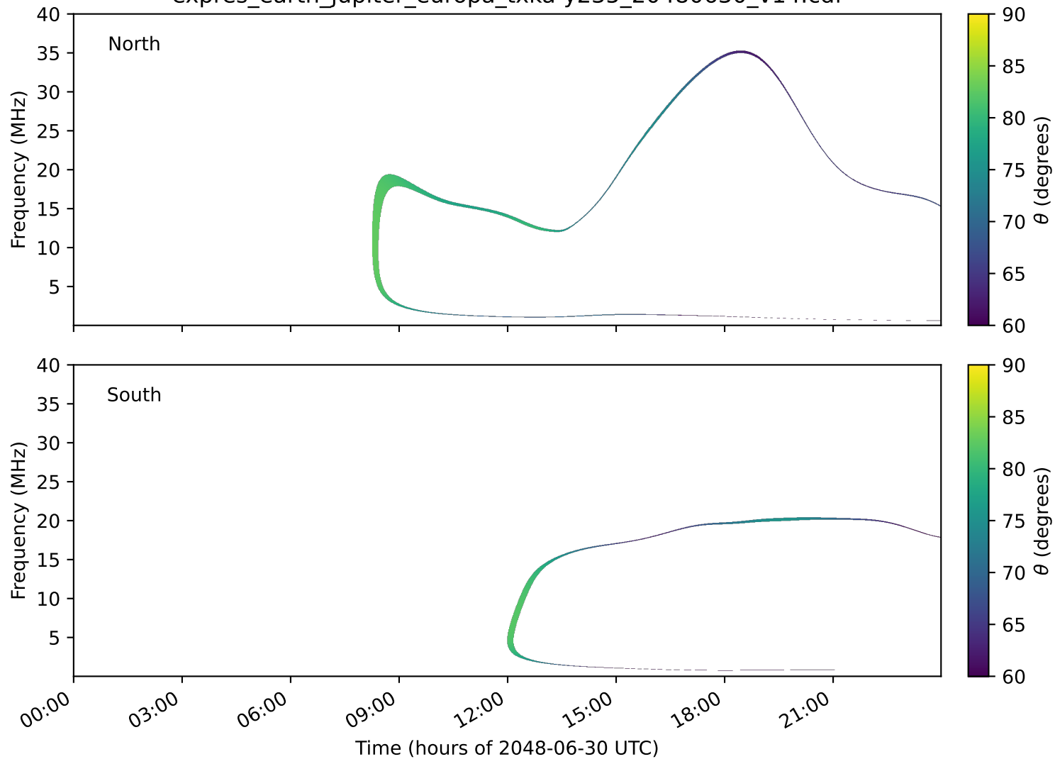
expres_earth_jupiter_europa_txka-y235_20480630_v14.cdf
