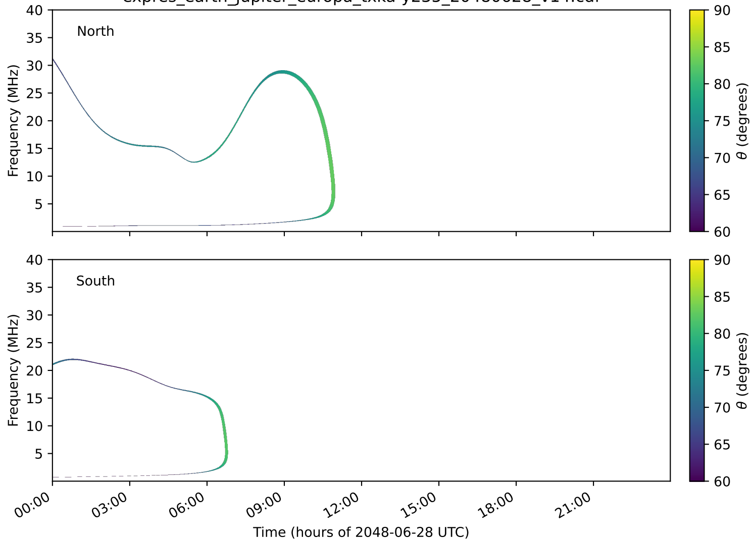
expres_earth_jupiter_europa_txka-y235_20480628_v14.cdf
