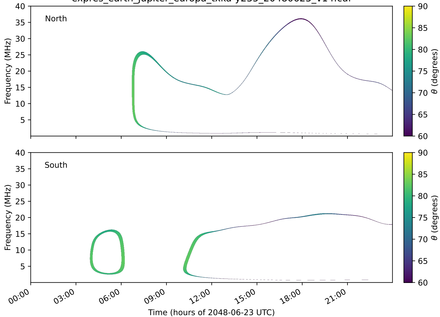
expres_earth_jupiter_europa_txka-y235_20480623_v14.cdf
