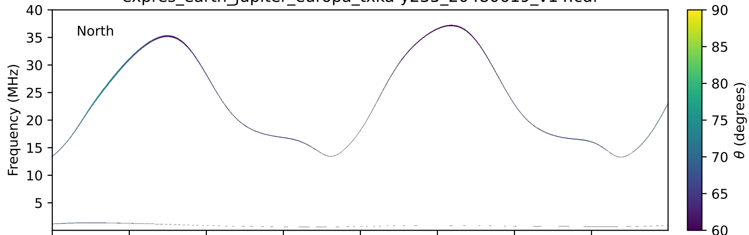
expres_earth_jupiter_europa_txka-y235_20480619_v14.cdf
