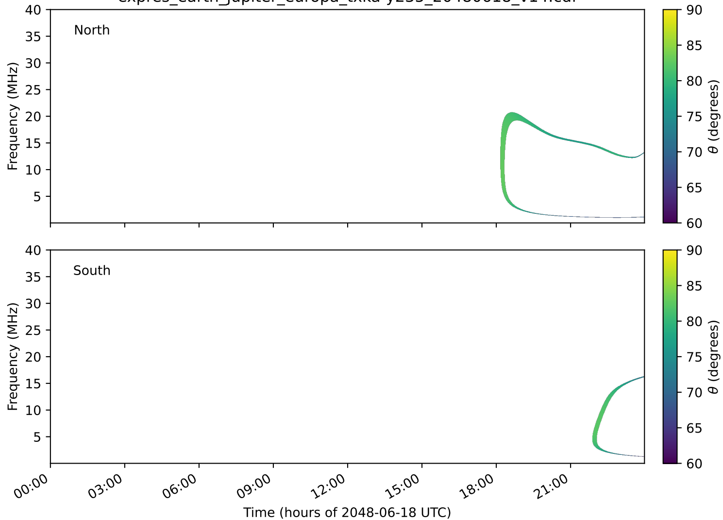
expres_earth_jupiter_europa_txka-y235_20480618_v14.cdf
