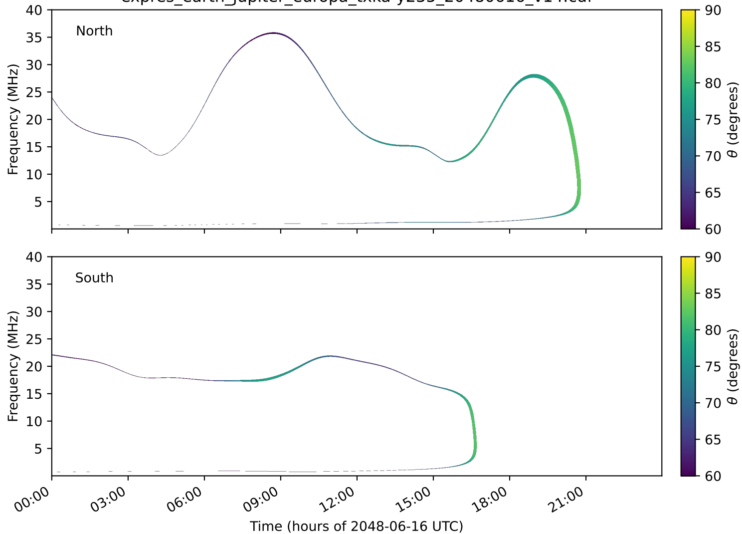
expres_earth_jupiter_europa_txka-y235_20480616_v14.cdf
