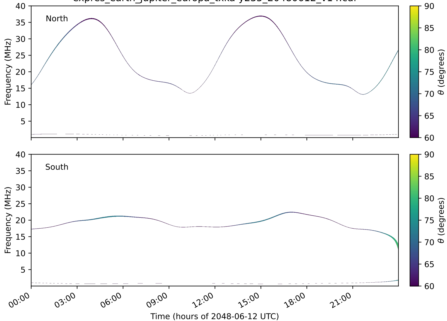
expres_earth_jupiter_europa_txka-y235_20480612_v14.cdf
