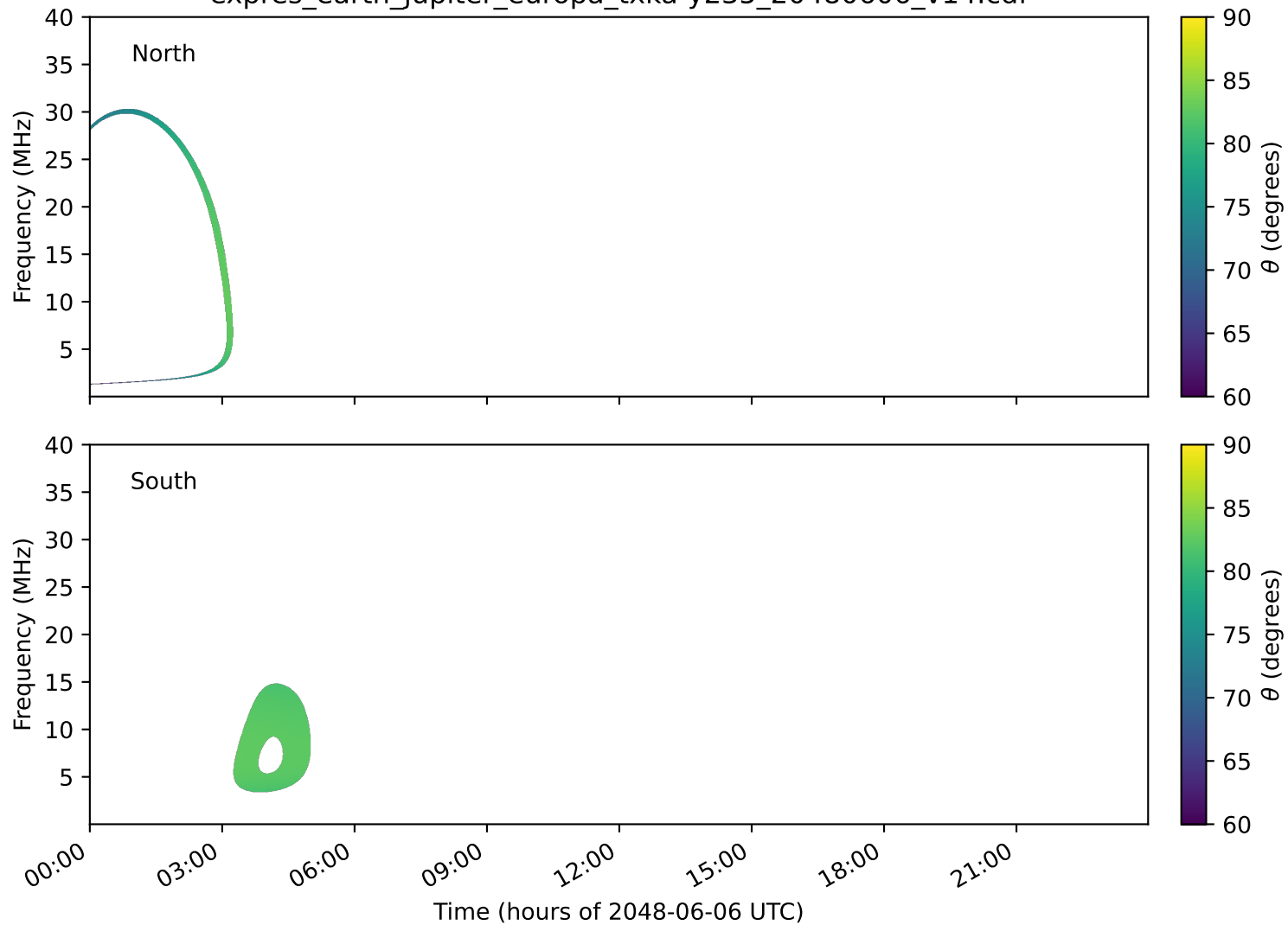
expres_earth_jupiter_europa_txka-y235_20480606_v14.cdf
