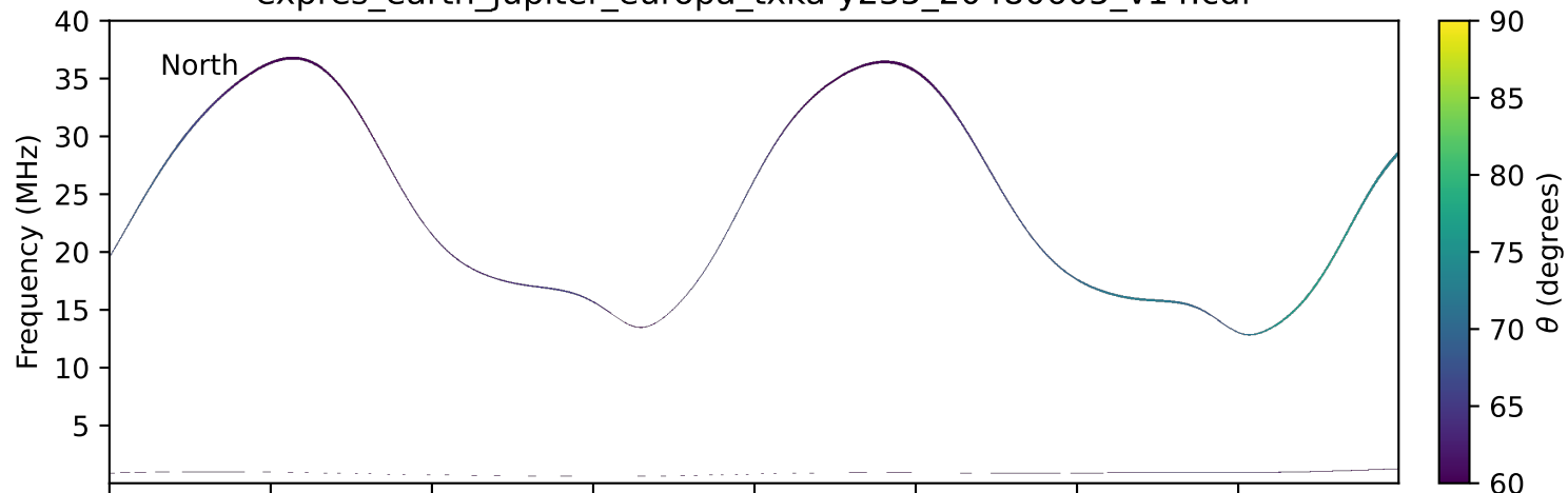
expres_earth_jupiter_europa_txka-y235_20480605_v14.cdf
