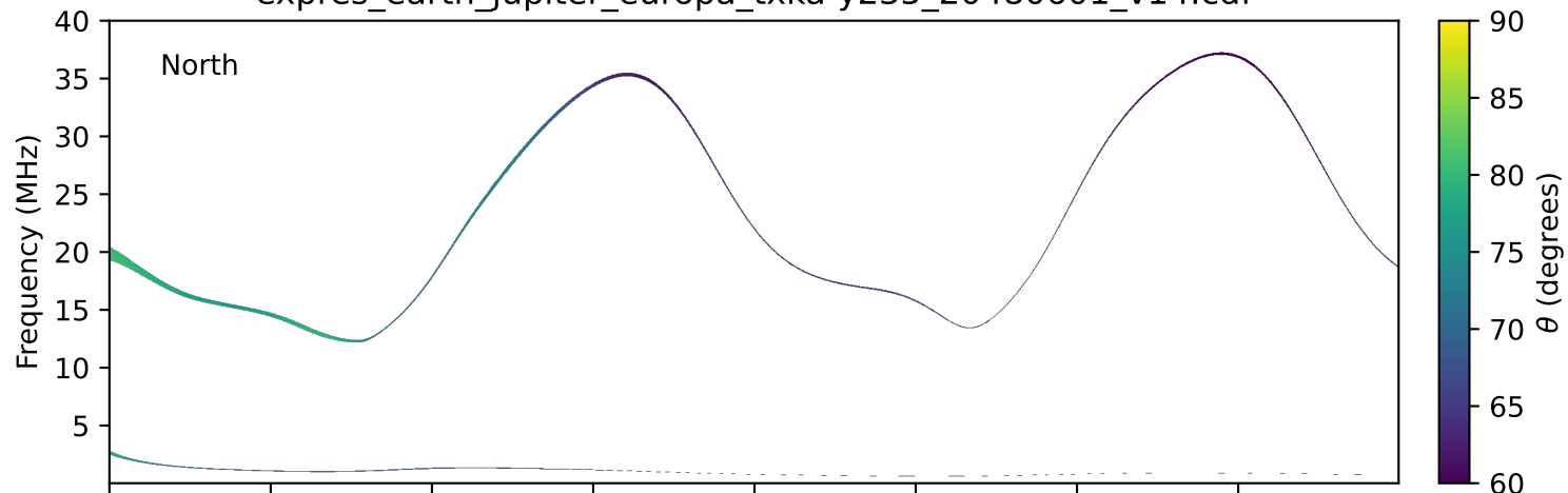
expres_earth_jupiter_europa_txka-y235_20480601_v14.cdf
