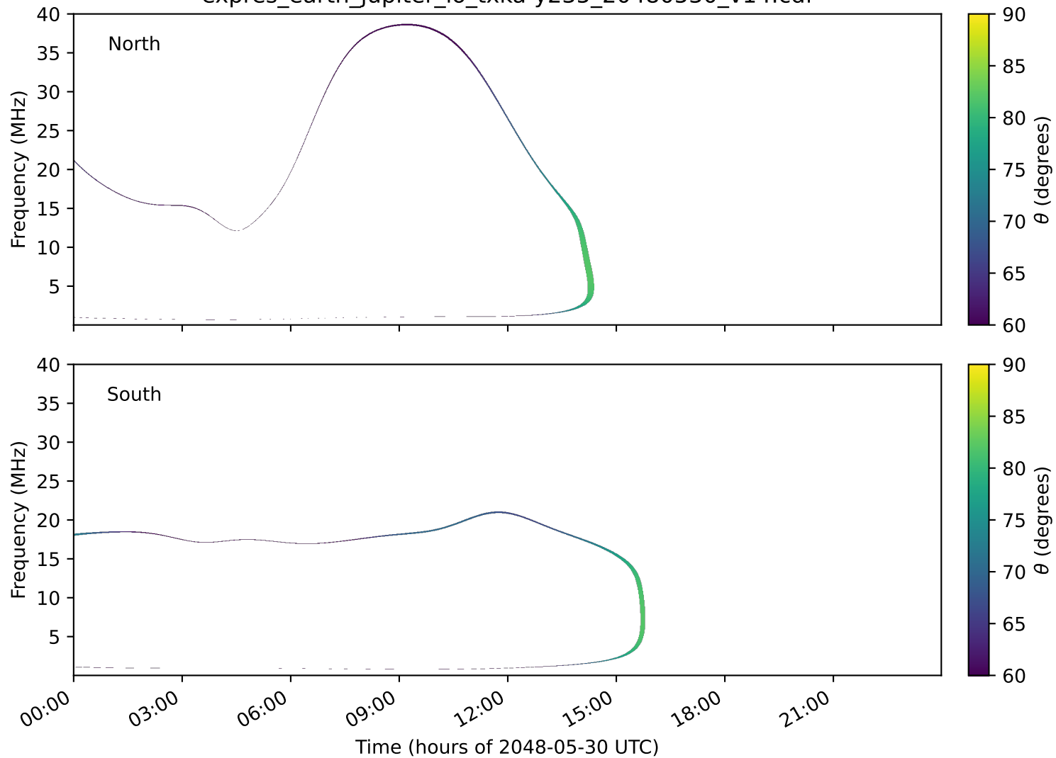
expres_earth_jupiter_io_txka-y235_20480530_v14.cdf
