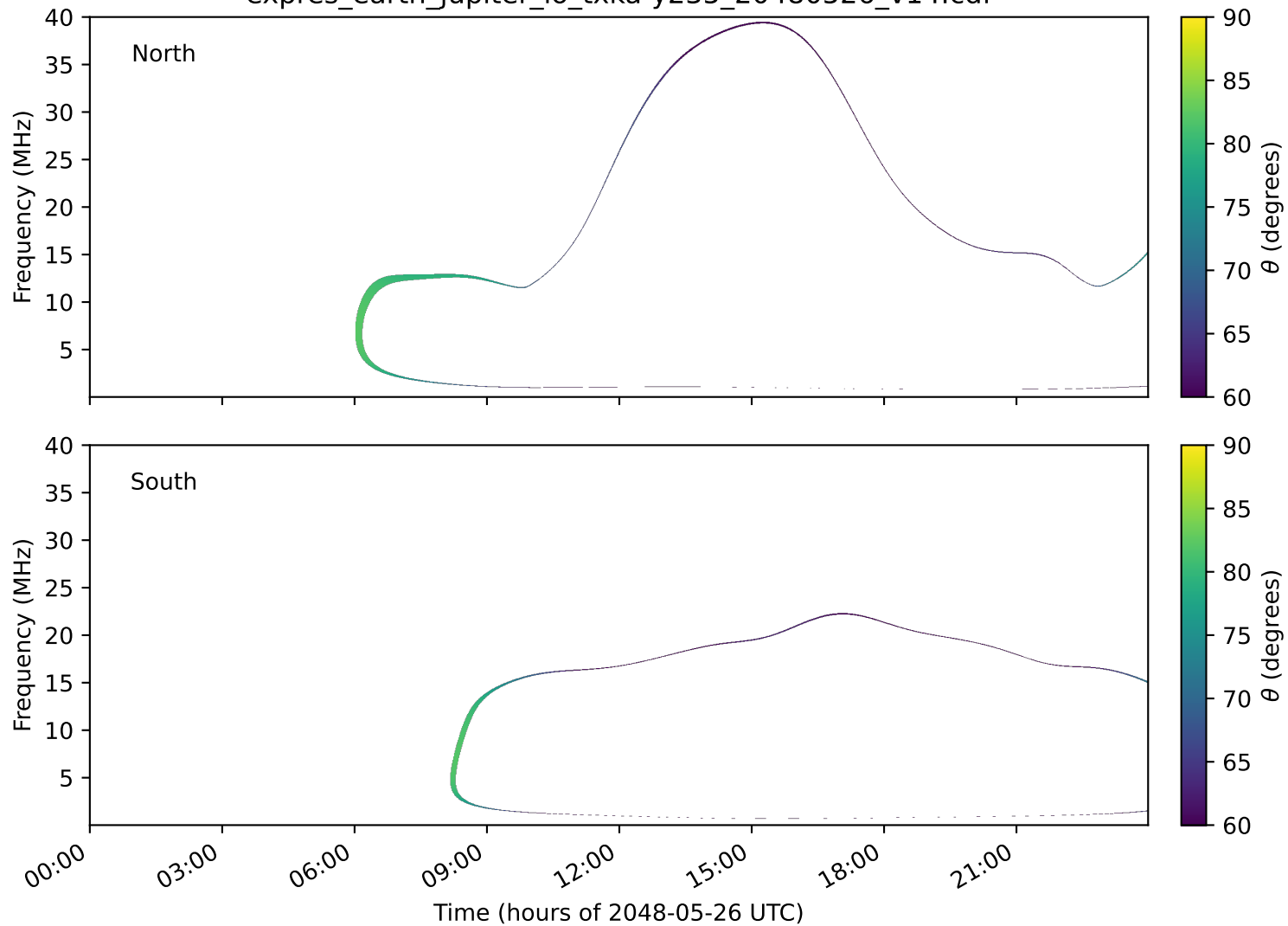
expres_earth_jupiter_io_txka-y235_20480526_v14.cdf
