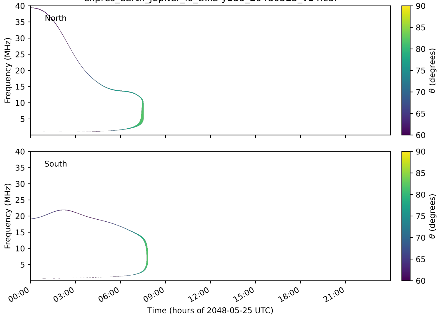
expres_earth_jupiter_io_txka-y235_20480525_v14.cdf
