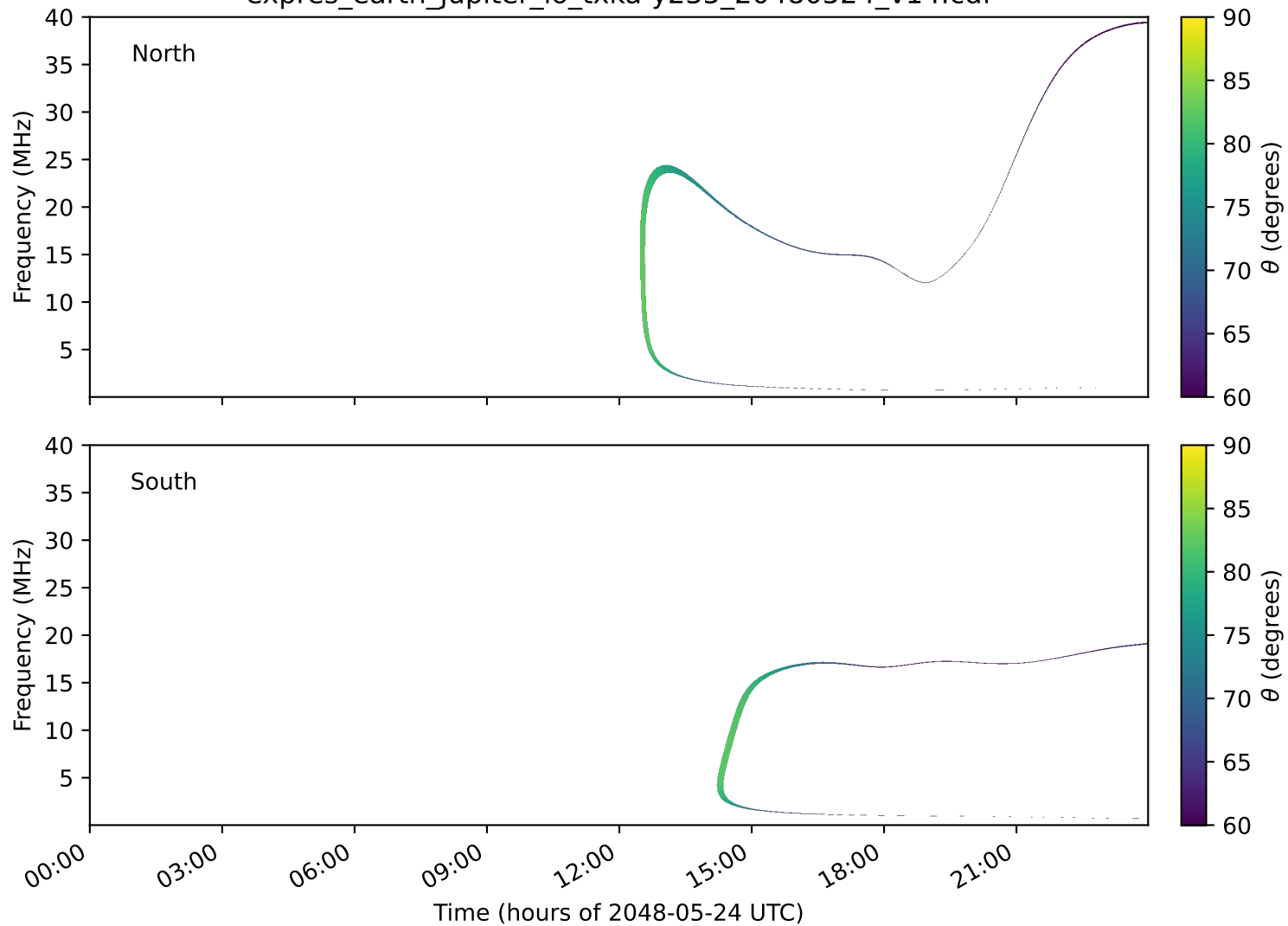
expres_earth_jupiter_io_txka-y235_20480524_v14.cdf
