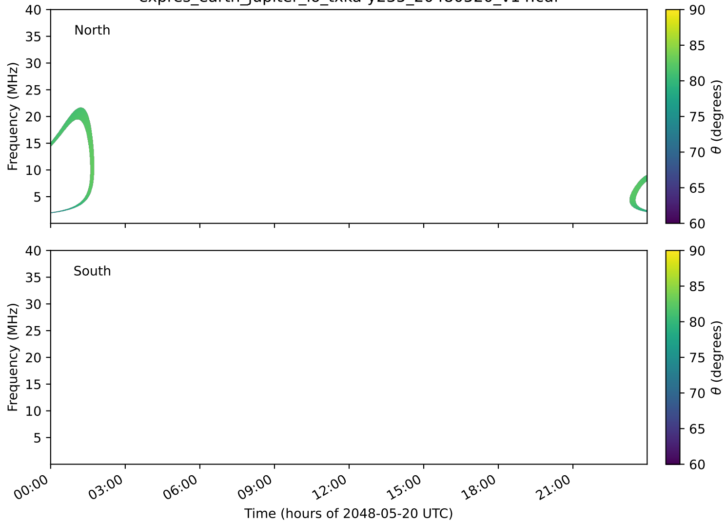
expres_earth_jupiter_io_txka-y235_20480520_v14.cdf
