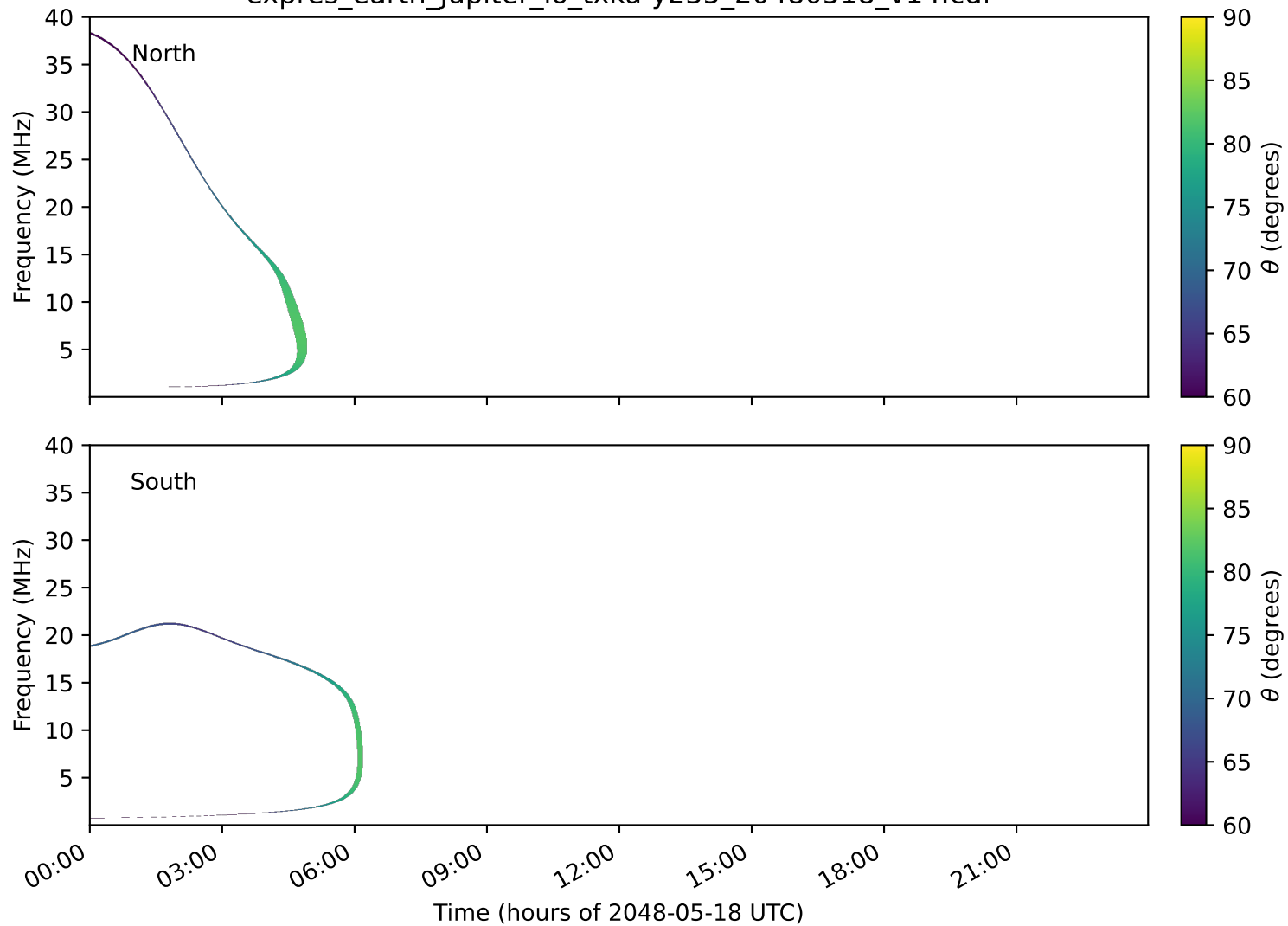
expres_earth_jupiter_io_txka-y235_20480518_v14.cdf
