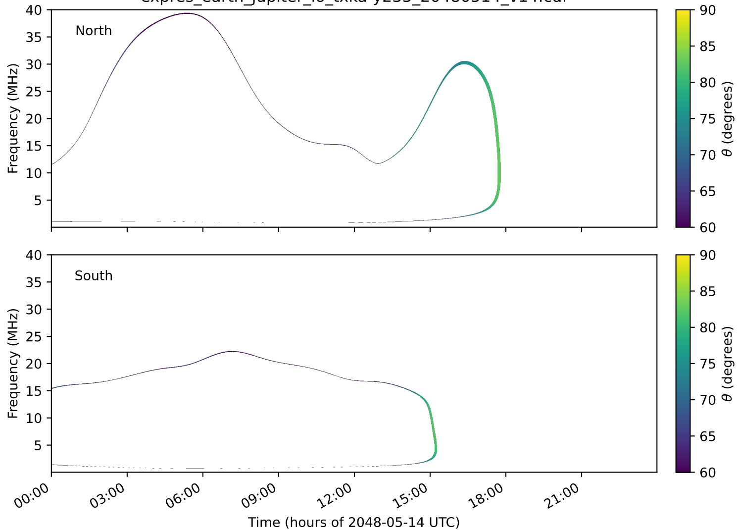
expres_earth_jupiter_io_txka-y235_20480514_v14.cdf
