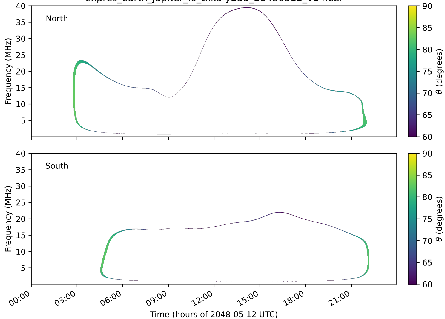
expres_earth_jupiter_io_txka-y235_20480512_v14.cdf
