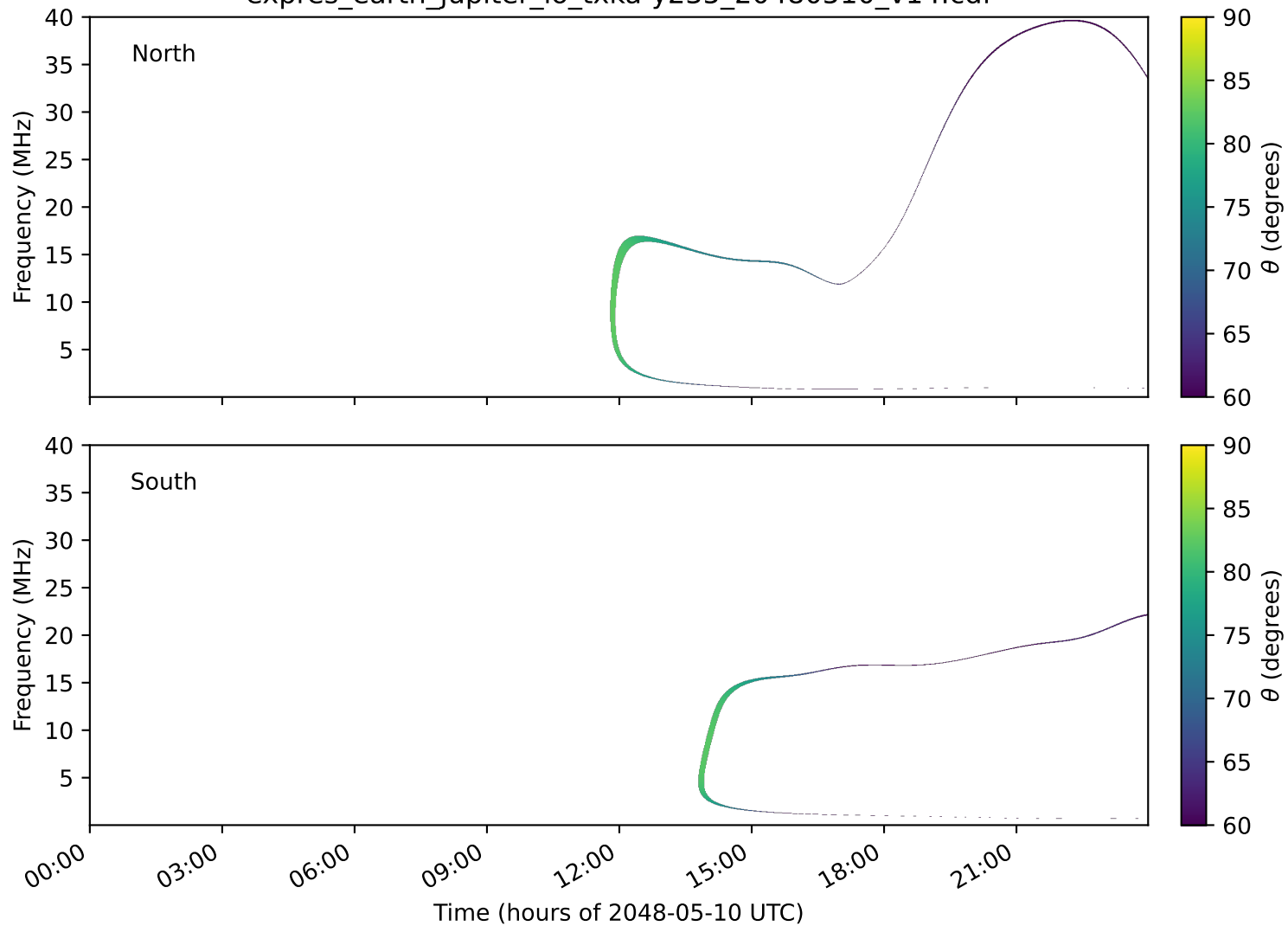
expres_earth_jupiter_io_txka-y235_20480510_v14.cdf
