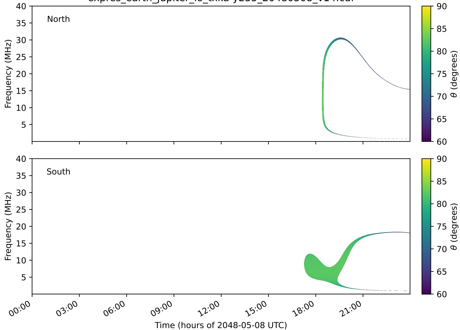
expres_earth_jupiter_io_txka-y235_20480508_v14.cdf
