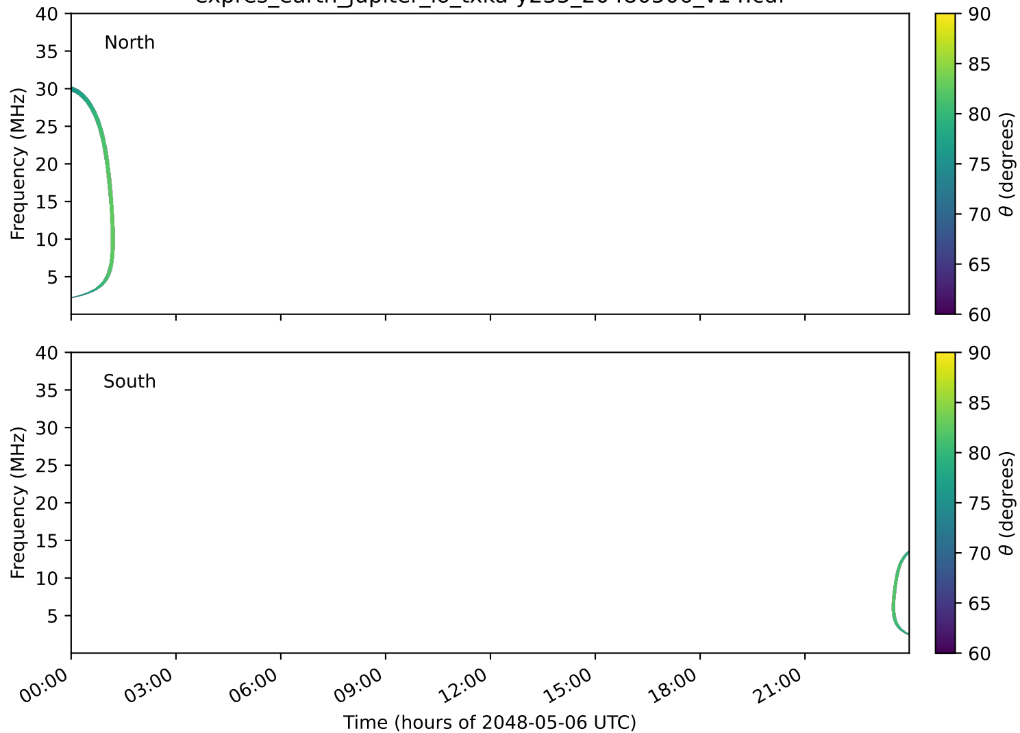
expres_earth_jupiter_io_txka-y235_20480506_v14.cdf
