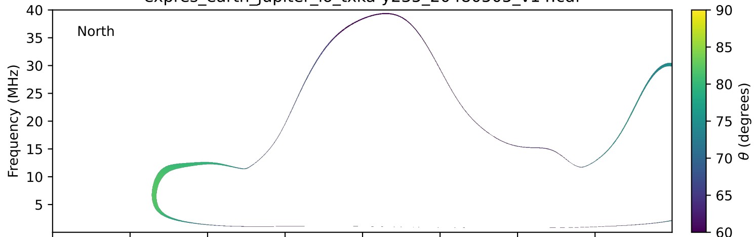
expres_earth_jupiter_io_txka-y235_20480505_v14.cdf
