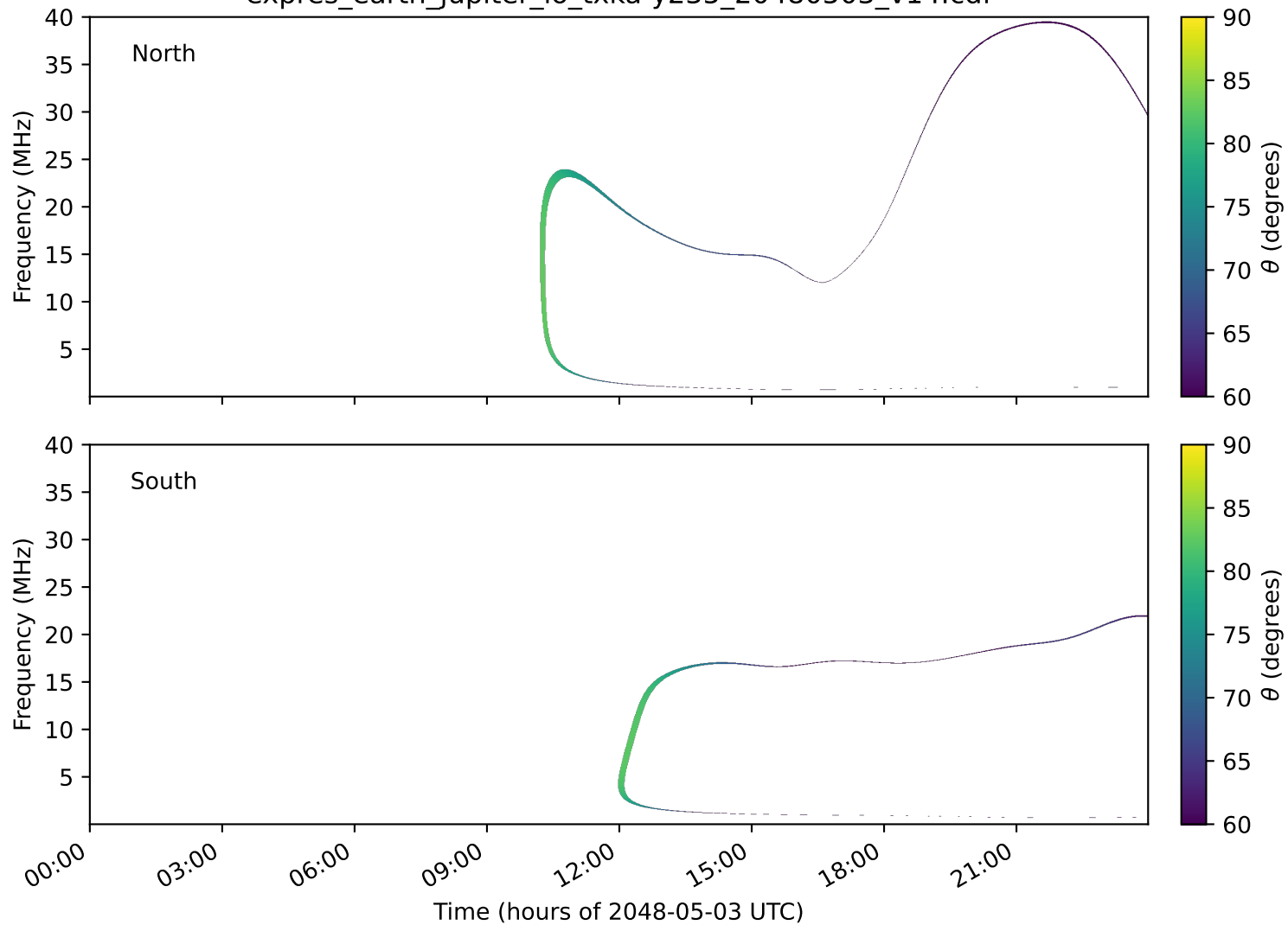
expres_earth_jupiter_io_txka-y235_20480503_v14.cdf
