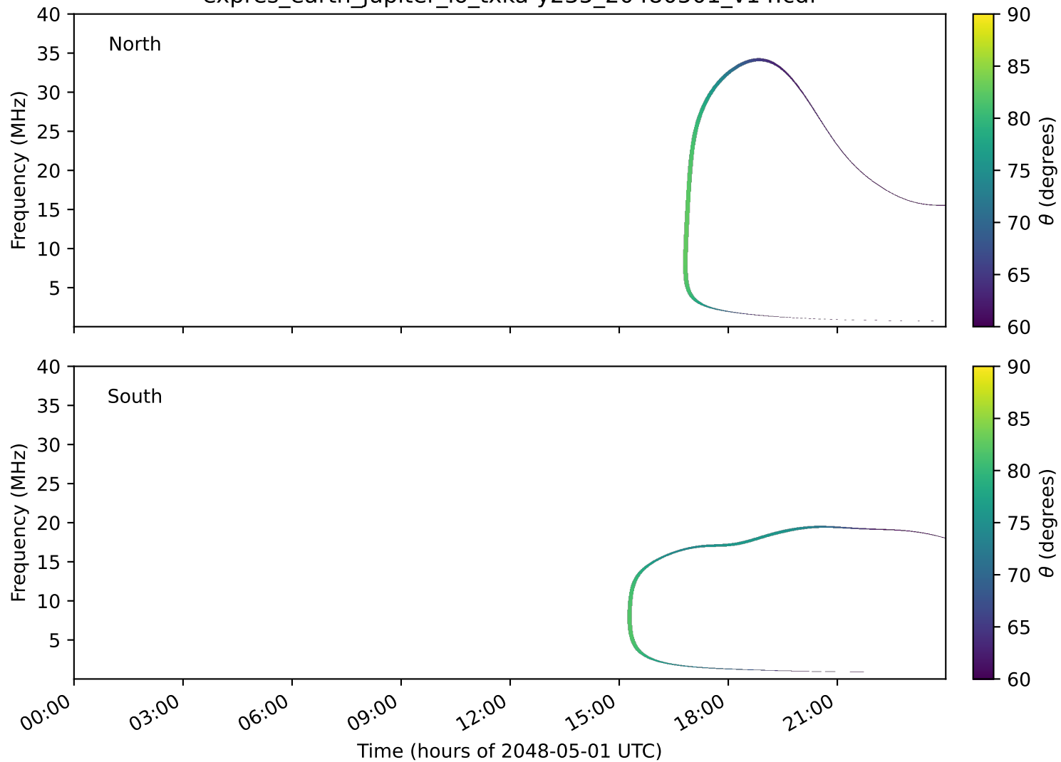
expres_earth_jupiter_io_txka-y235_20480501_v14.cdf
