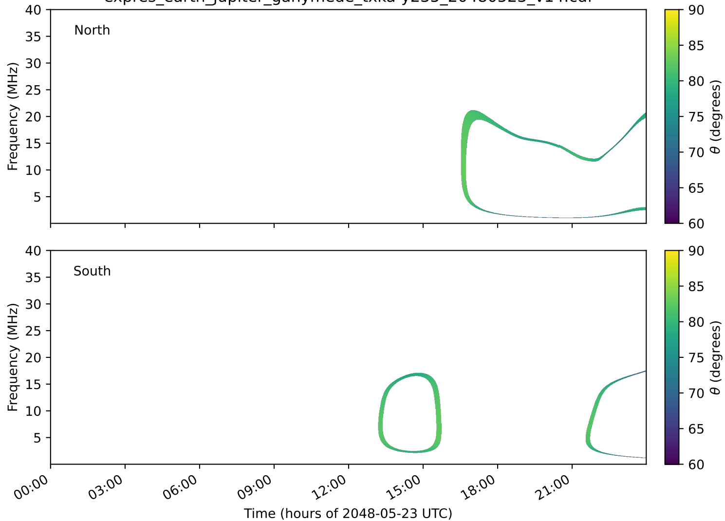
expres_earth_jupiter_ganymede_txka-y235_20480523_v14.cdf
