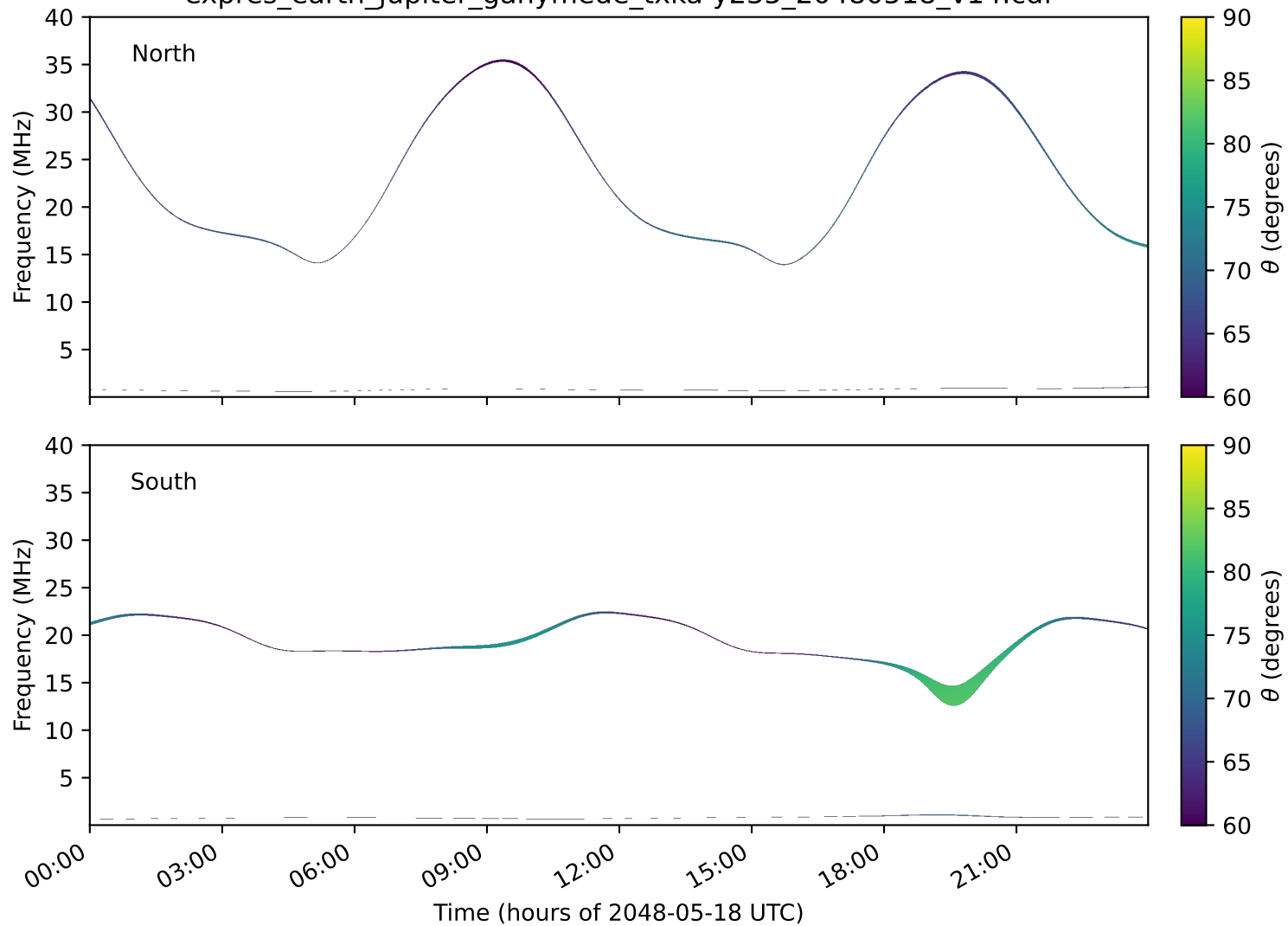
expres_earth_jupiter_ganymede_txka-y235_20480518_v14.cdf
