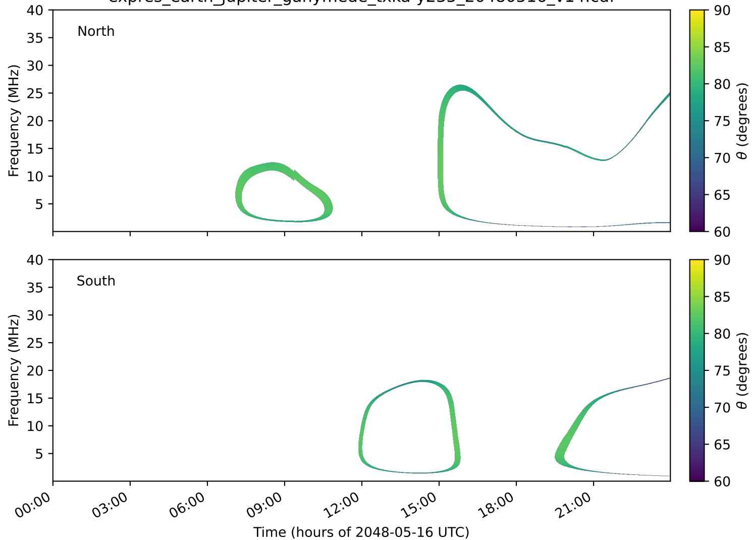
expres_earth_jupiter_ganymede_txka-y235_20480516_v14.cdf
