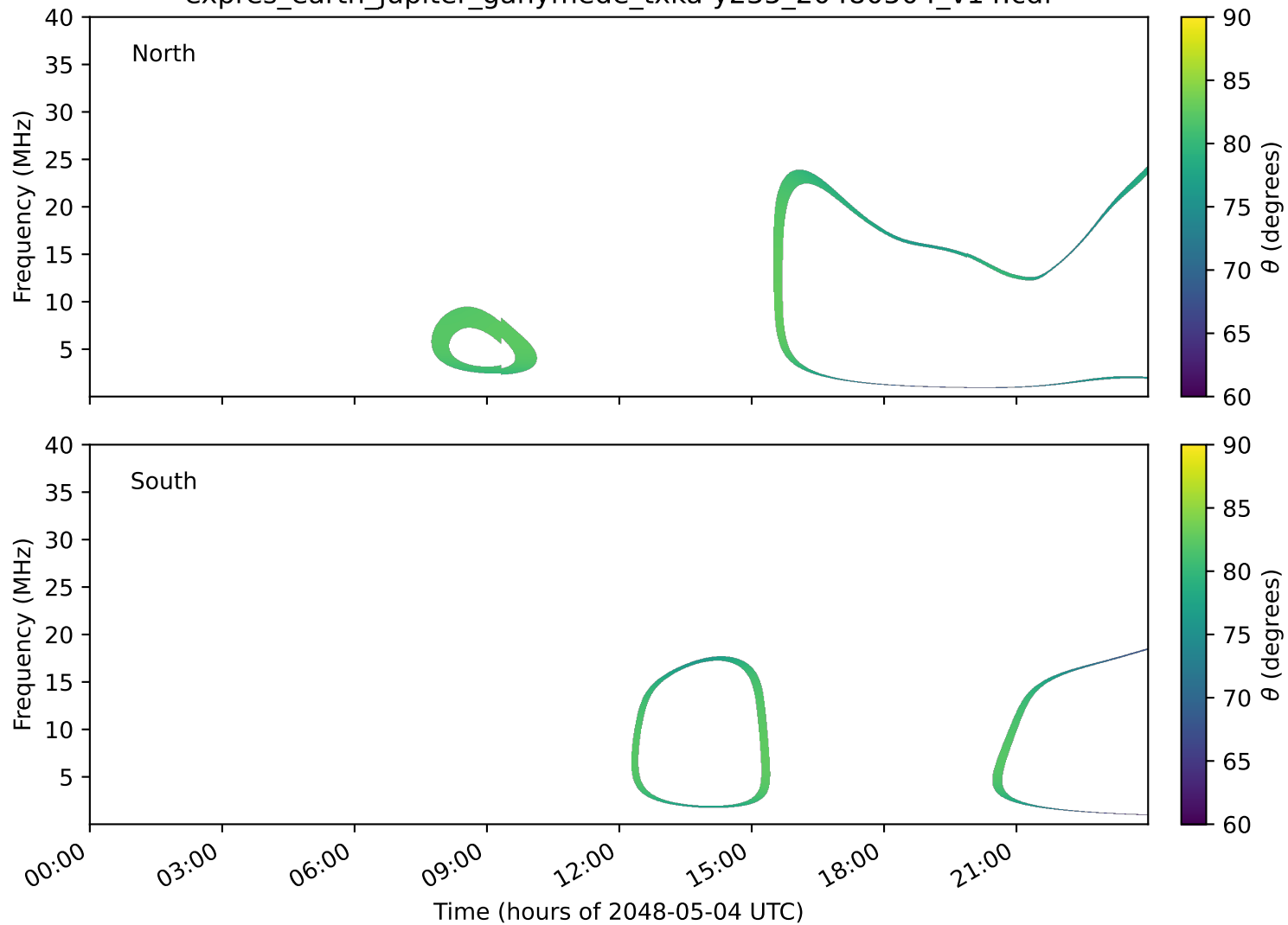
expres_earth_jupiter_ganymede_txka-y235_20480504_v14.cdf
