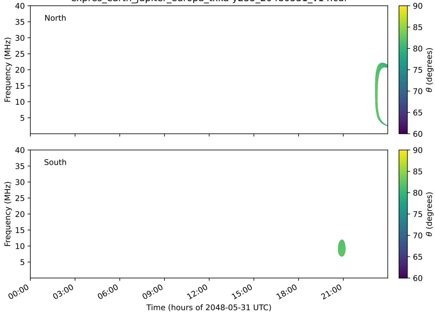
expres_earth_jupiter_europa_txka-y235_20480531_v14.cdf
