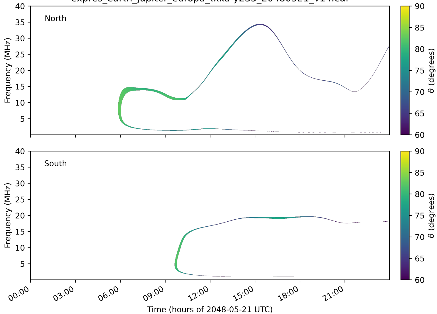
expres_earth_jupiter_europa_txka-y235_20480521_v14.cdf
