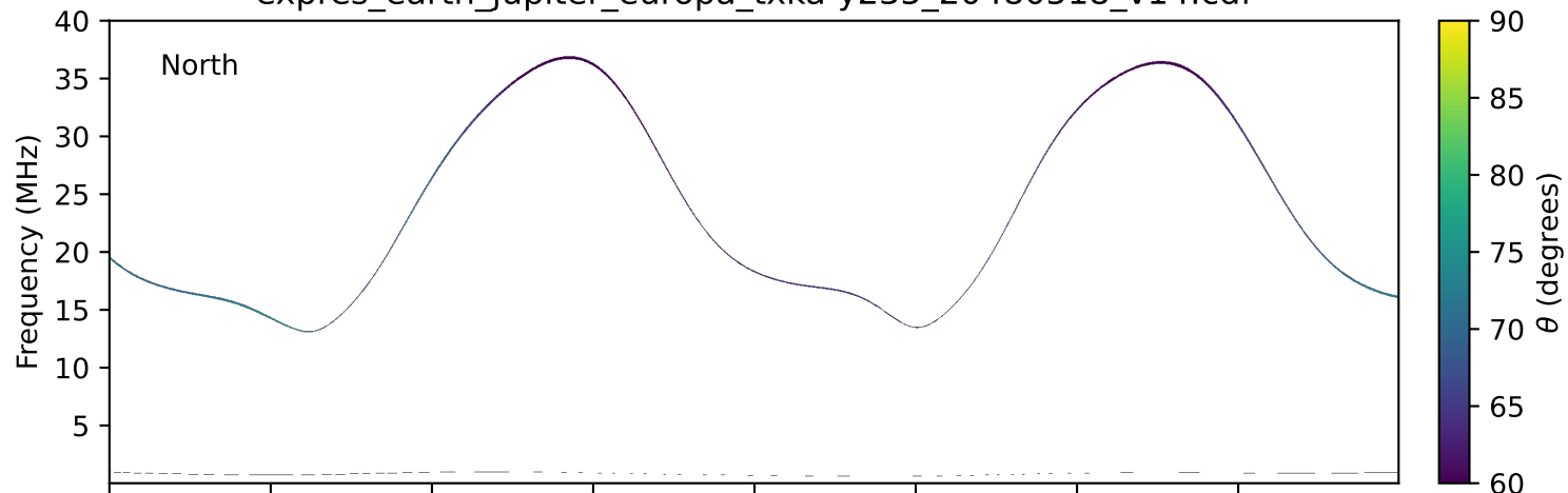
expres_earth_jupiter_europa_txka-y235_20480518_v14.cdf
