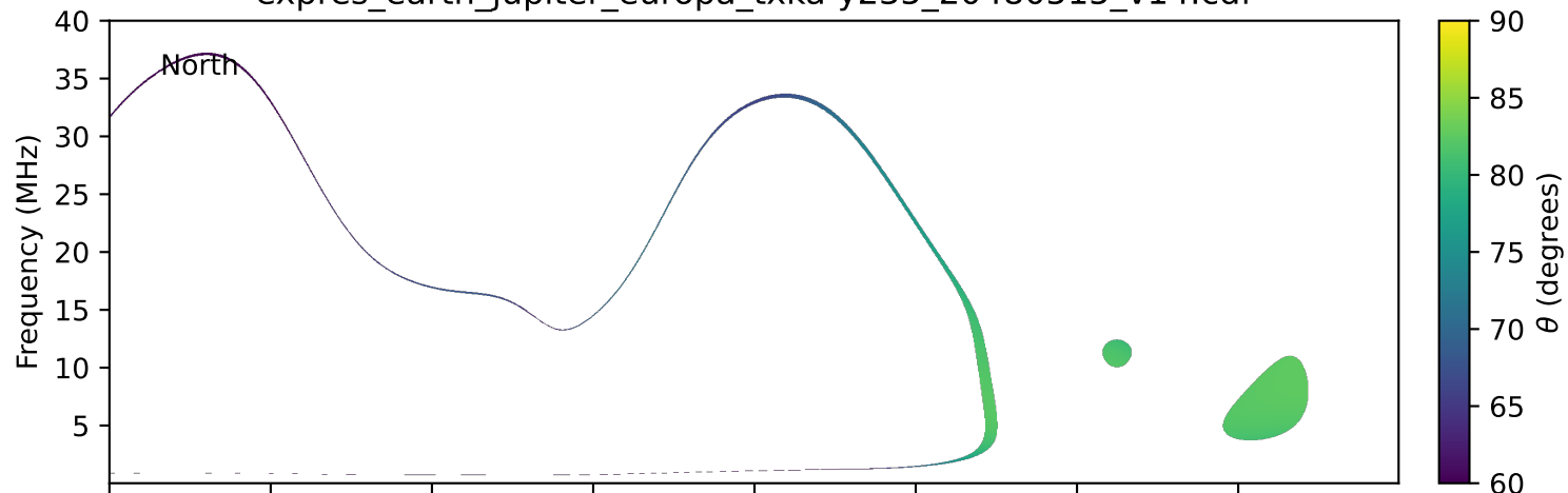
expres_earth_jupiter_europa_txka-y235_20480515_v14.cdf
