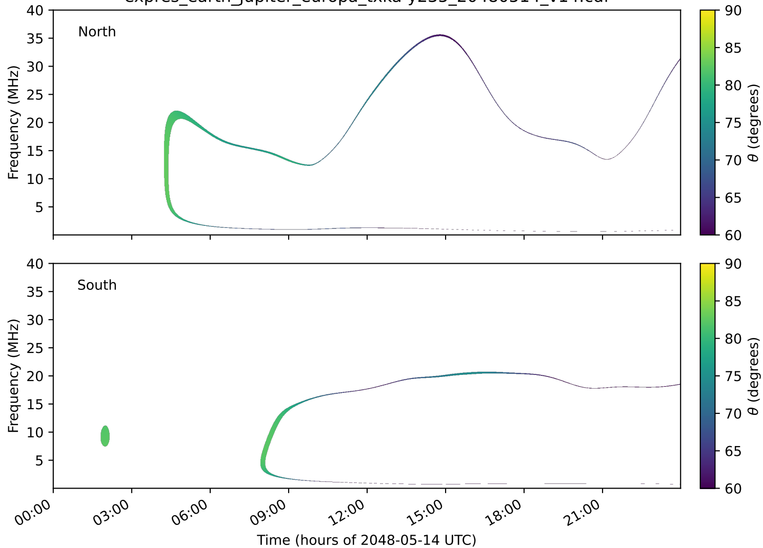
expres_earth_jupiter_europa_txka-y235_20480514_v14.cdf
