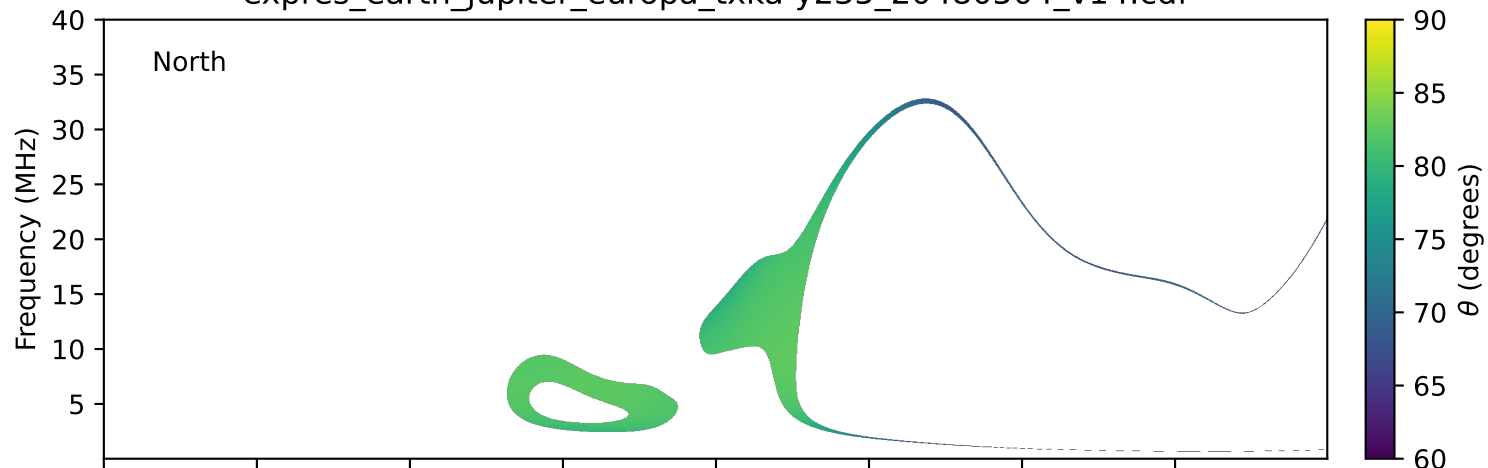
expres_earth_jupiter_europa_txka-y235_20480504_v14.cdf
