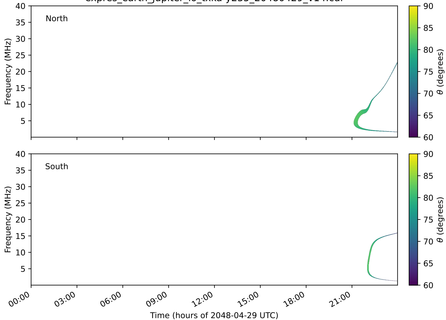
expres_earth_jupiter_io_txka-y235_20480429_v14.cdf
