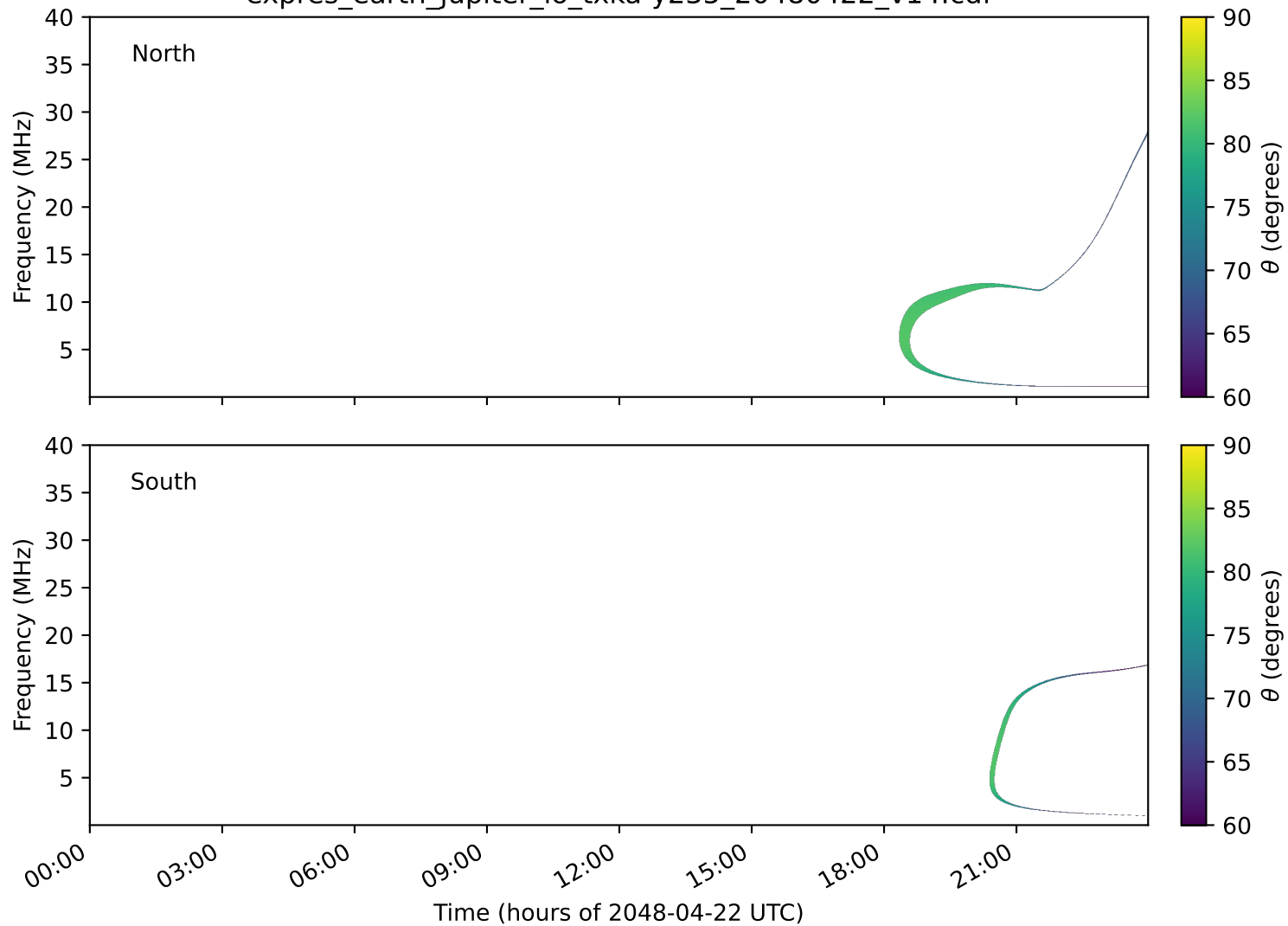
expres_earth_jupiter_io_txka-y235_20480422_v14.cdf
