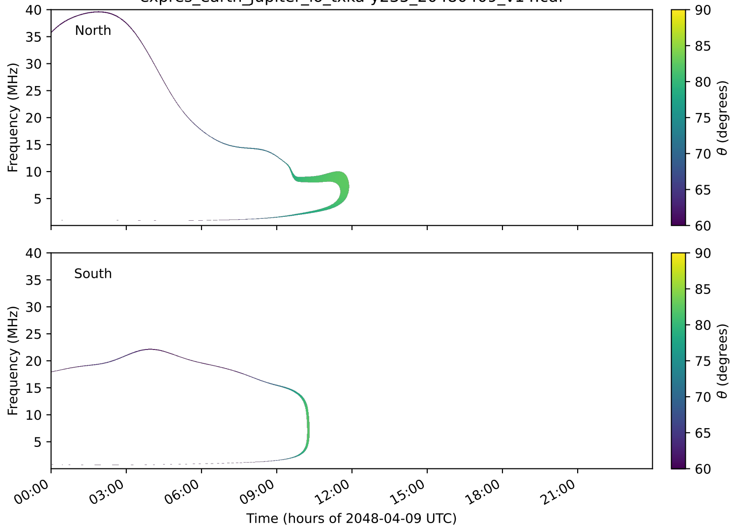
expres_earth_jupiter_io_txka-y235_20480409_v14.cdf
