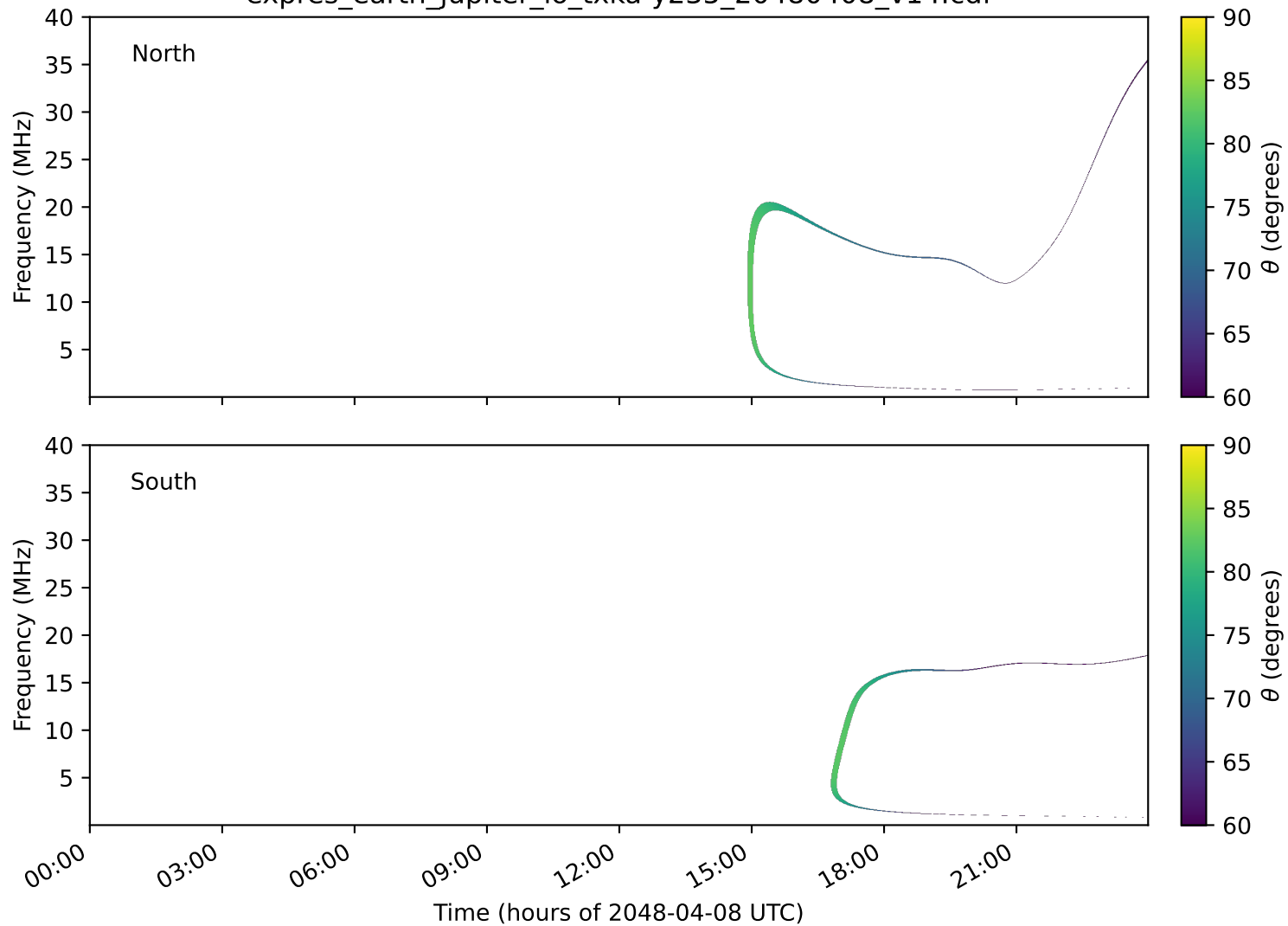
expres_earth_jupiter_io_txka-y235_20480408_v14.cdf
